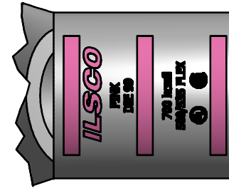
DETAIL B TOP AND BOTTOM INK MARKINGS ARE IDENTICAL INK COLOR: PINK
